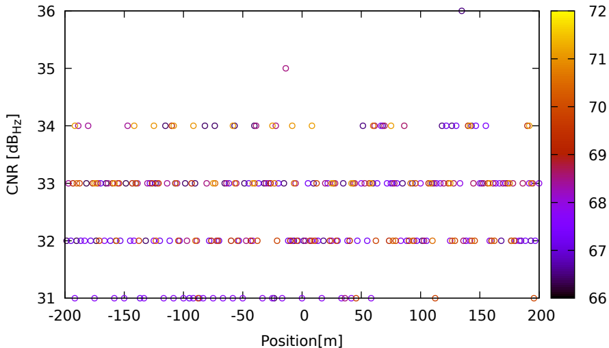
CNR vs position for G03 (L5) on HuaweiP40 - DOY 262 jam. 2
