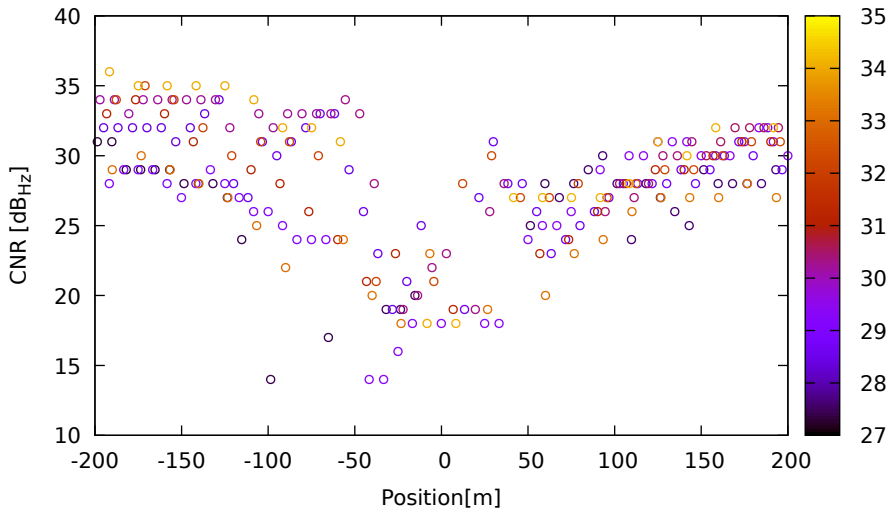
CNR vs position for G04 (L1) on HuaweiP40 - DOY 262 jam. 2
