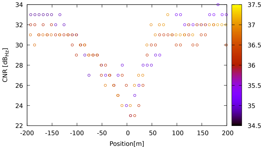
CNR vs position for G04 (L1) on HuaweiP40 - DOY 262 jam. 3
