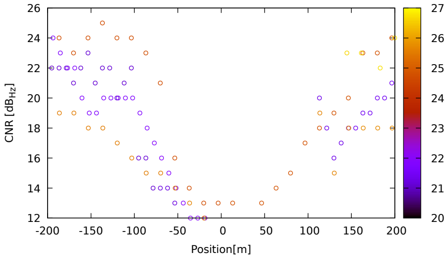
CNR vs position for G04 (L5) on HuaweiP40 - DOY 262 jam. 1
