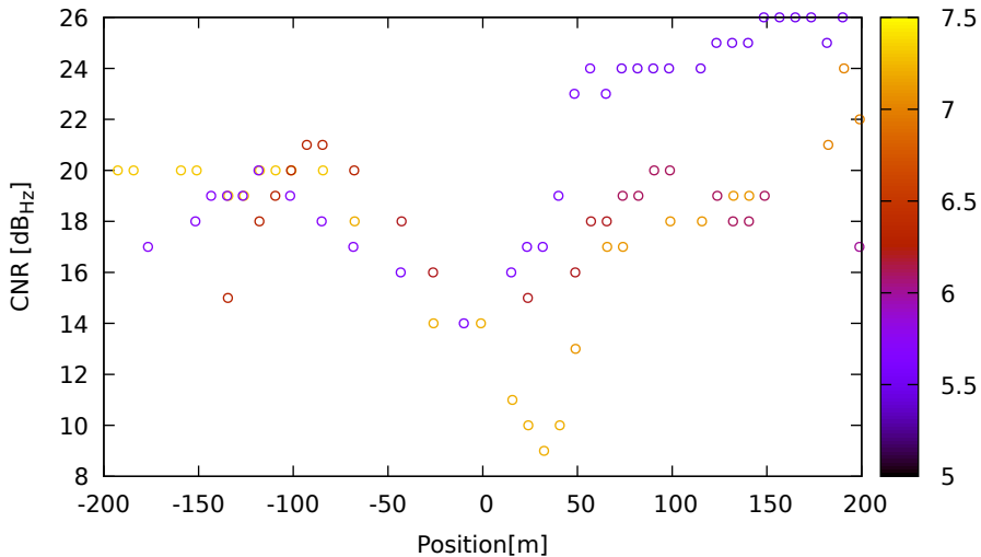
CNR vs position for G08 (L1) on HuaweiP40 - DOY 262 jam. 3
