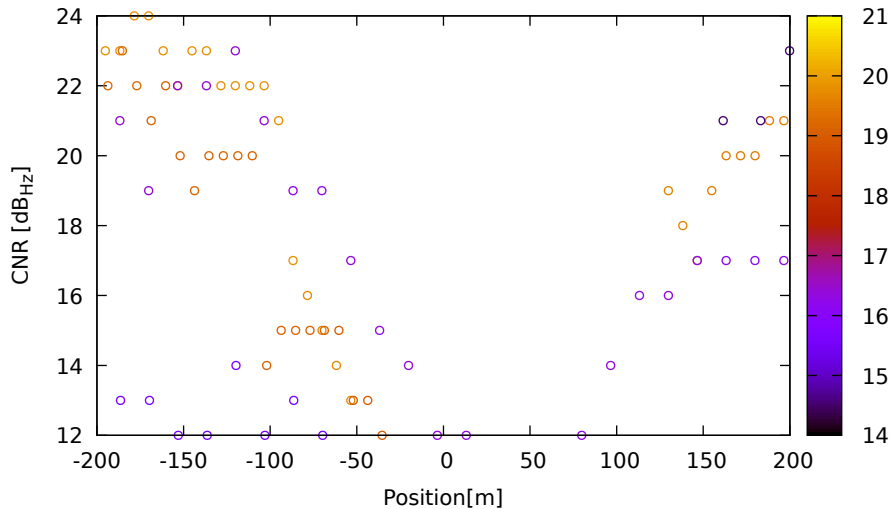
CNR vs position for G08 (L5) on HuaweiP40 - DOY 262 jam. 1
