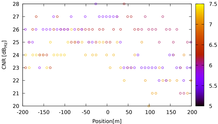
CNR vs position for G08 (L5) on HuaweiP40 - DOY 262 jam. 3
