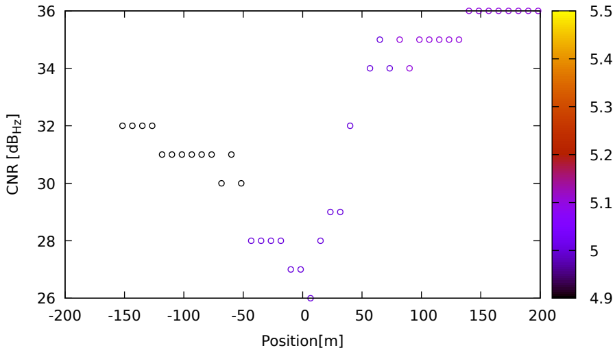
CNR vs position for G09 (L1) on HuaweiP40 - DOY 262 jam. 3
