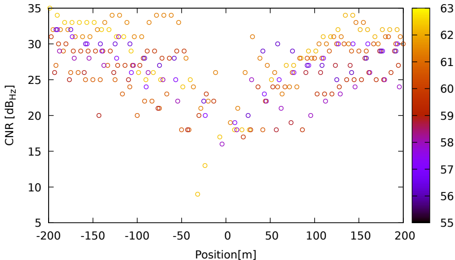
CNR vs position for G21 (L1) on HuaweiP40 - DOY 262 jam. 2
