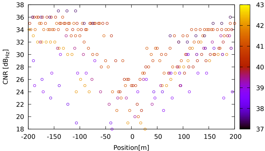
CNR vs position for G22 (L1) on HuaweiP40 - DOY 262 jam. 2
