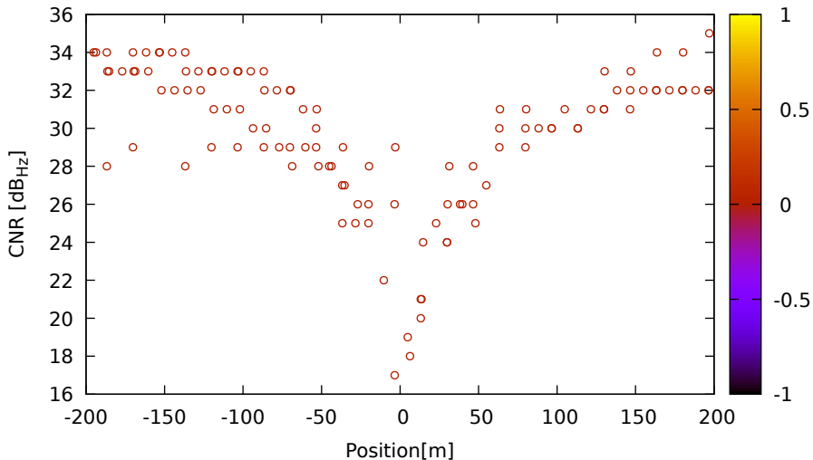
CNR vs position for G28 (L1) on HuaweiP40 - DOY 262 jam. 1
