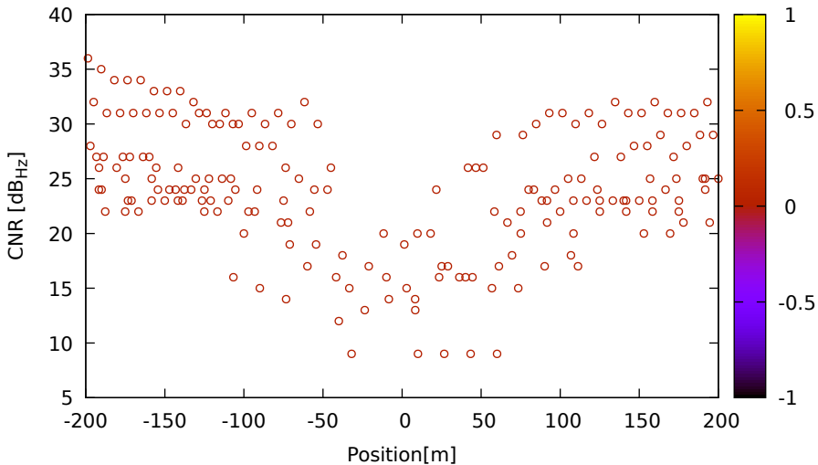
CNR vs position for G28 (L1) on HuaweiP40 - DOY 262 jam. 2
