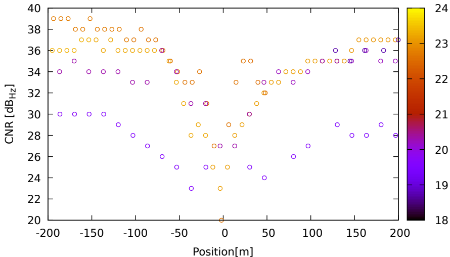
CNR vs position for G32 (L1) on HuaweiP40 - DOY 262 jam. 1
