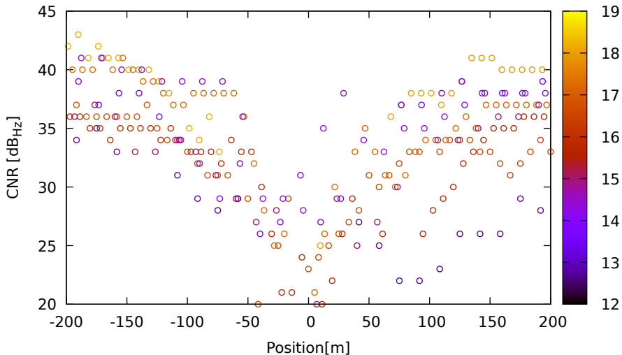
CNR vs position for G32 (L1) on HuaweiP40 - DOY 262 jam. 2
