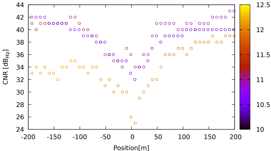
CNR vs position for G32 (L1) on HuaweiP40 - DOY 262 jam. 3
