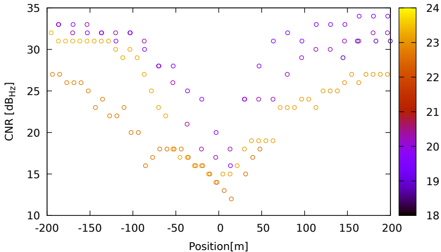
CNR vs position for G32 (L5) on HuaweiP40 - DOY 262 jam. 1
