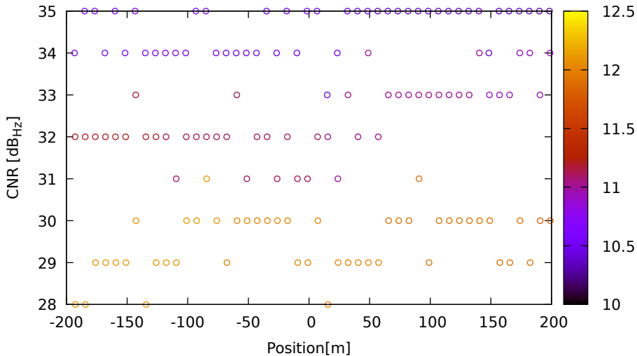
CNR vs position for G32 (L5) on HuaweiP40 - DOY 262 jam. 3
