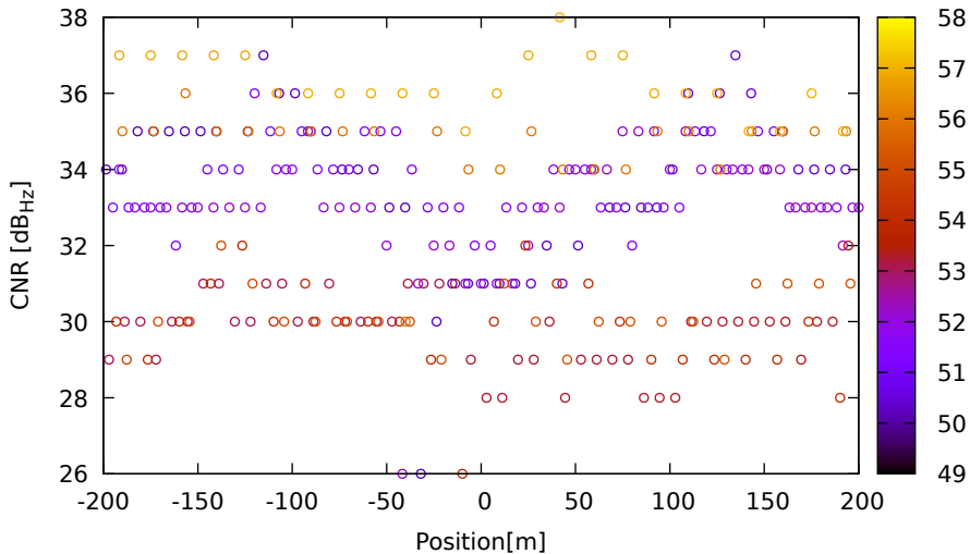
CNR vs position for R01 (G1) on HuaweiP40 - DOY 262 jam. 2
