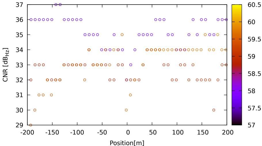
CNR vs position for R01 (G1) on HuaweiP40 - DOY 262 jam. 3
