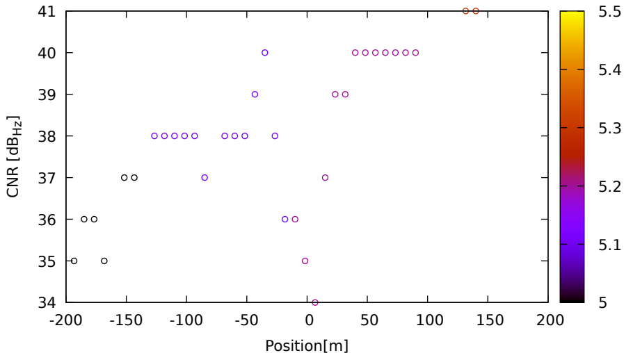
CNR vs position for R02 (G1) on HuaweiP40 - DOY 262 jam. 3
