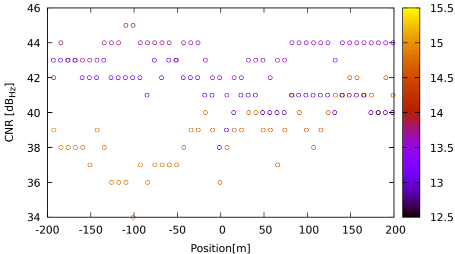
CNR vs position for R07 (G1) on HuaweiP40 - DOY 262 jam. 3
