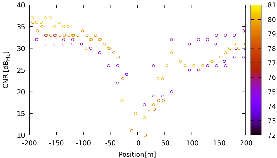
CNR vs position for R08 (G1) on HuaweiP40 - DOY 262 jam. 1
