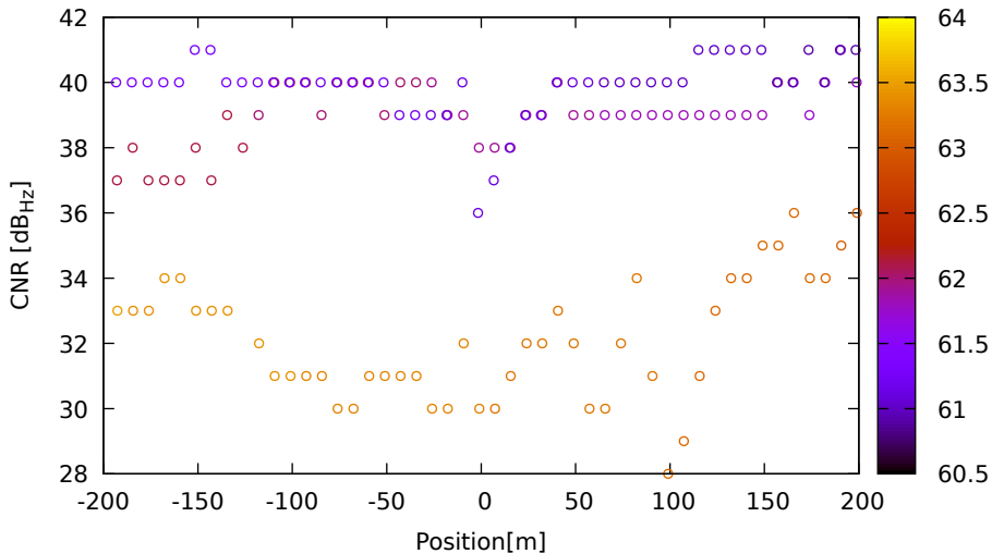
CNR vs position for R08 (G1) on HuaweiP40 - DOY 262 jam. 3
