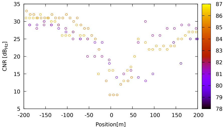
CNR vs position for R23 (G1) on HuaweiP40 - DOY 262 jam. 1
