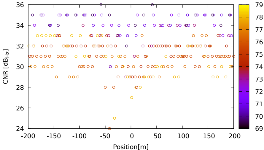
CNR vs position for R23 (G1) on HuaweiP40 - DOY 262 jam. 2
