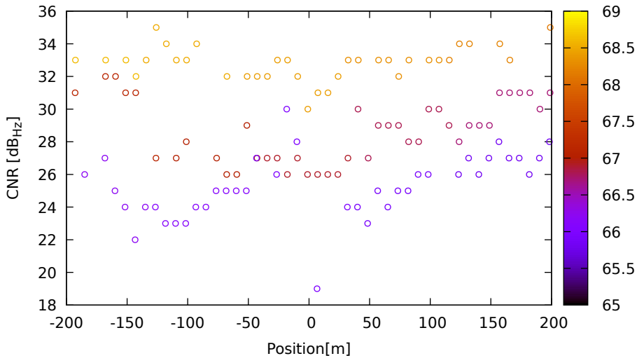
CNR vs position for R23 (G1) on HuaweiP40 - DOY 262 jam. 3
