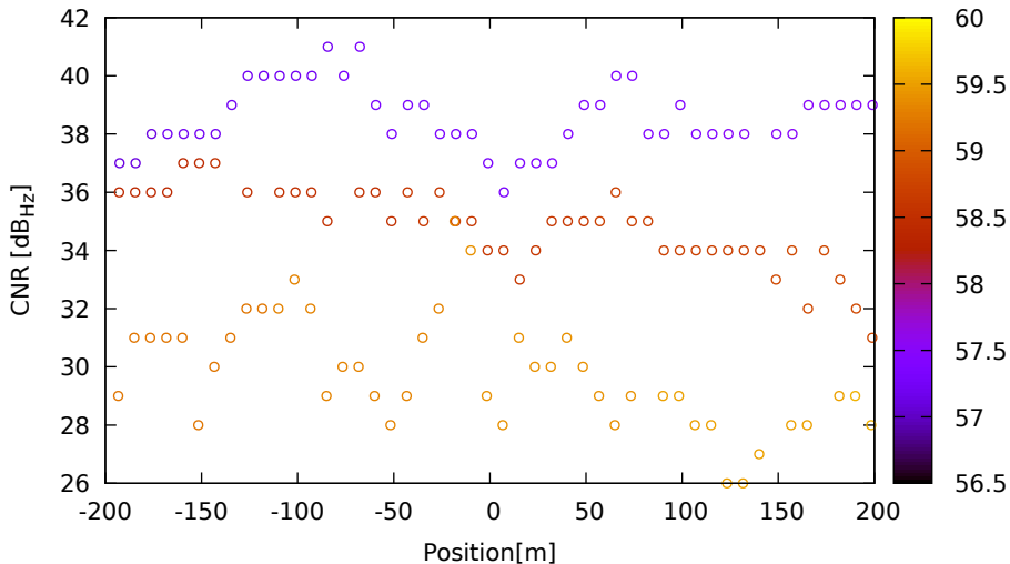
CNR vs position for R24 (G1) on HuaweiP40 - DOY 262 jam. 3
