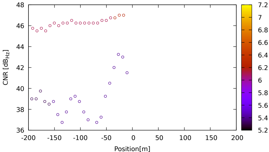
CNR vs position for E03 (E5b) on LeicaGS15 - DOY 262 jam. 3
