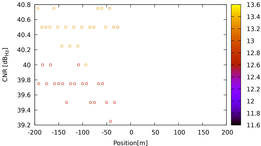
CNR vs position for E04 (E5) on LeicaGS15 - DOY 262 jam. 3
