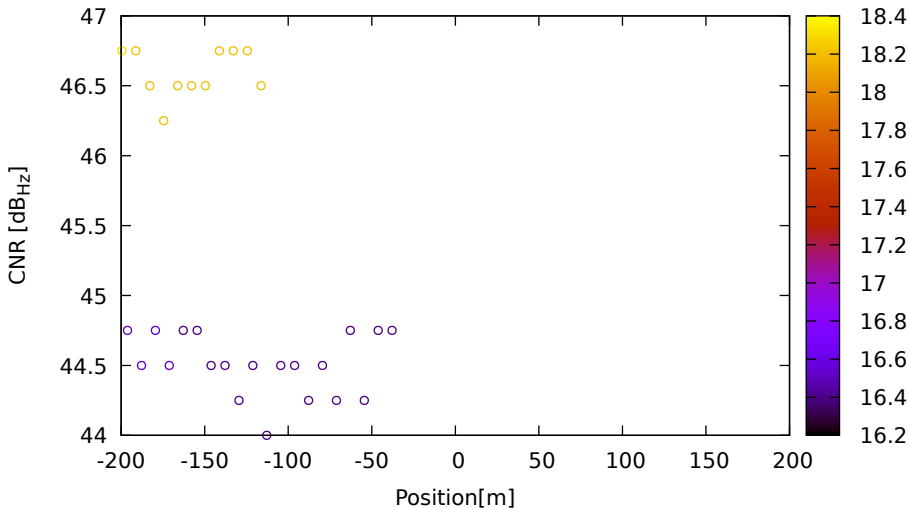
CNR vs position for E04 (E5b) on LeicaGS15 - DOY 262 jam. 2
