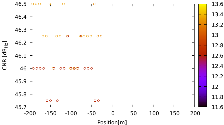
CNR vs position for E04 (E5b) on LeicaGS15 - DOY 262 jam. 3
