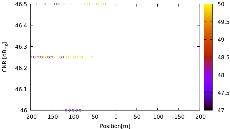
CNR vs position for E05 (E5) on LeicaGS15 - DOY 262 jam. 2
