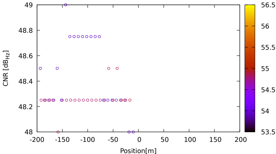
CNR vs position for E05 (E5a) on LeicaGS15 - DOY 262 jam. 3
