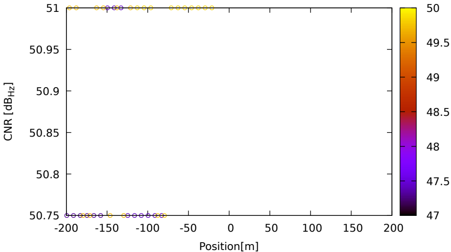
CNR vs position for E05 (E5b) on LeicaGS15 - DOY 262 jam. 2
