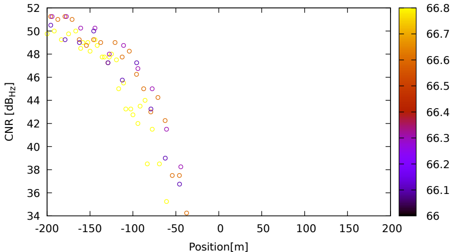
CNR vs position for E09 (E1) on LeicaGS15 - DOY 262 jam. 1
