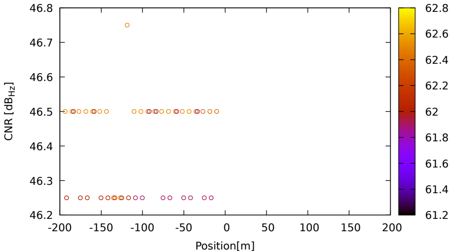
CNR vs position for E09 (E5) on LeicaGS15 - DOY 262 jam. 3
