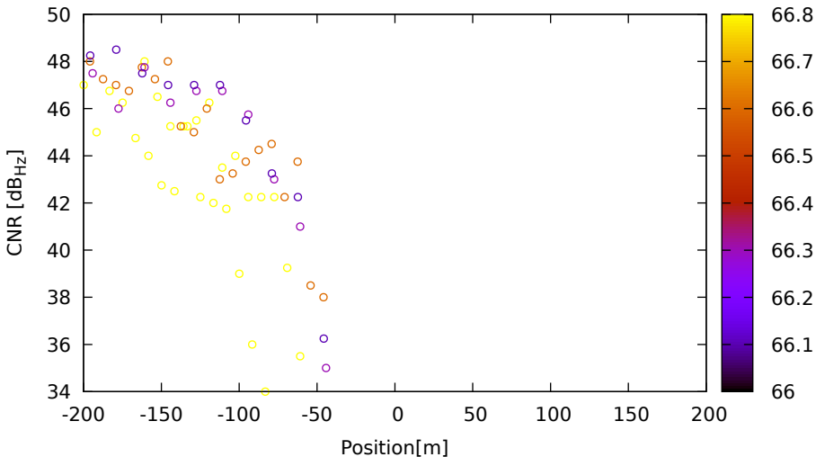
CNR vs position for E09 (E5a) on LeicaGS15 - DOY 262 jam. 1
