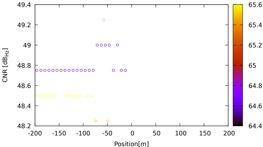
CNR vs position for E09 (E5a) on LeicaGS15 - DOY 262 jam. 2
