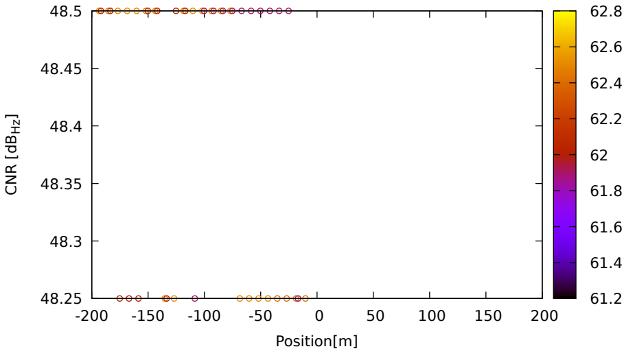
CNR vs position for E09 (E5a) on LeicaGS15 - DOY 262 jam. 3
