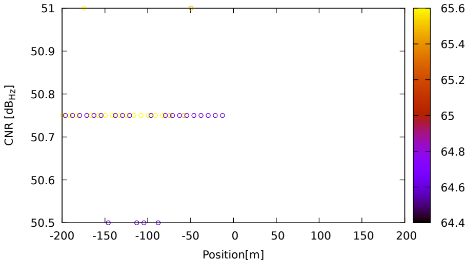
CNR vs position for E09 (E5b) on LeicaGS15 - DOY 262 jam. 2
