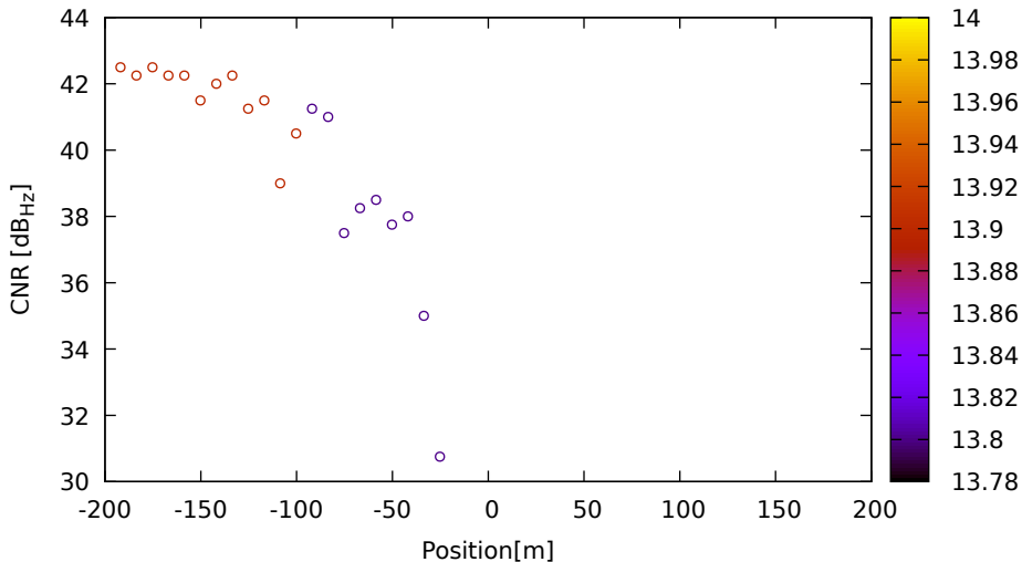
CNR vs position for E11 (E1) on LeicaGS15 - DOY 262 jam. 3
