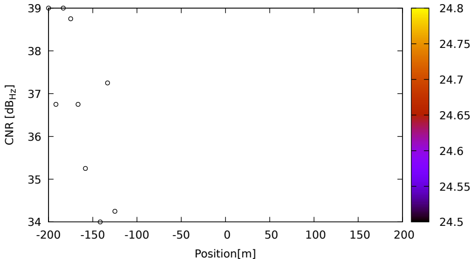
CNR vs position for E11 (E5a) on LeicaGS15 - DOY 262 jam. 1
