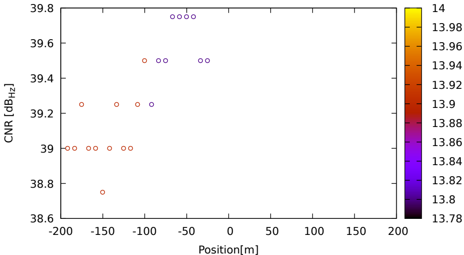
CNR vs position for E11 (E5a) on LeicaGS15 - DOY 262 jam. 3
