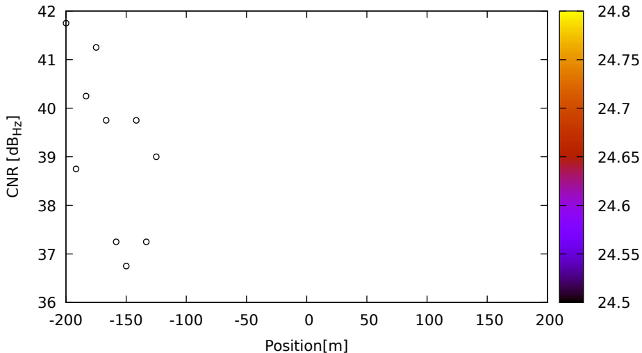
CNR vs position for E11 (E5b) on LeicaGS15 - DOY 262 jam. 1
