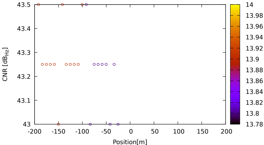
CNR vs position for E11 (E5b) on LeicaGS15 - DOY 262 jam. 3
