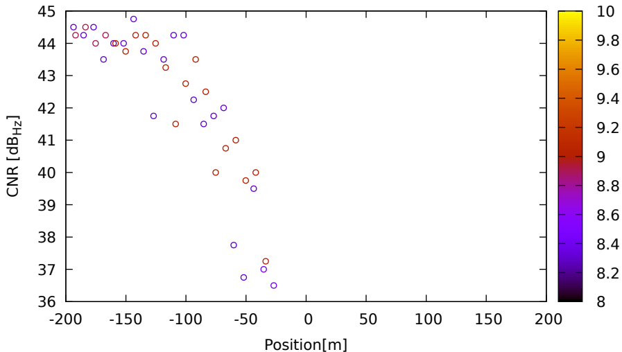
CNR vs position for E15 (E1) on LeicaGS15 - DOY 262 jam. 3
