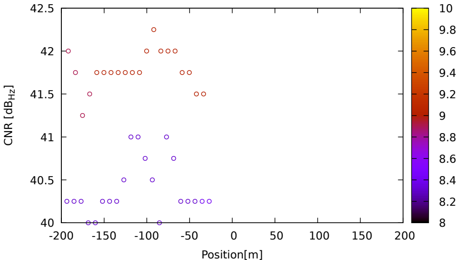
CNR vs position for E15 (E5a) on LeicaGS15 - DOY 262 jam. 3
