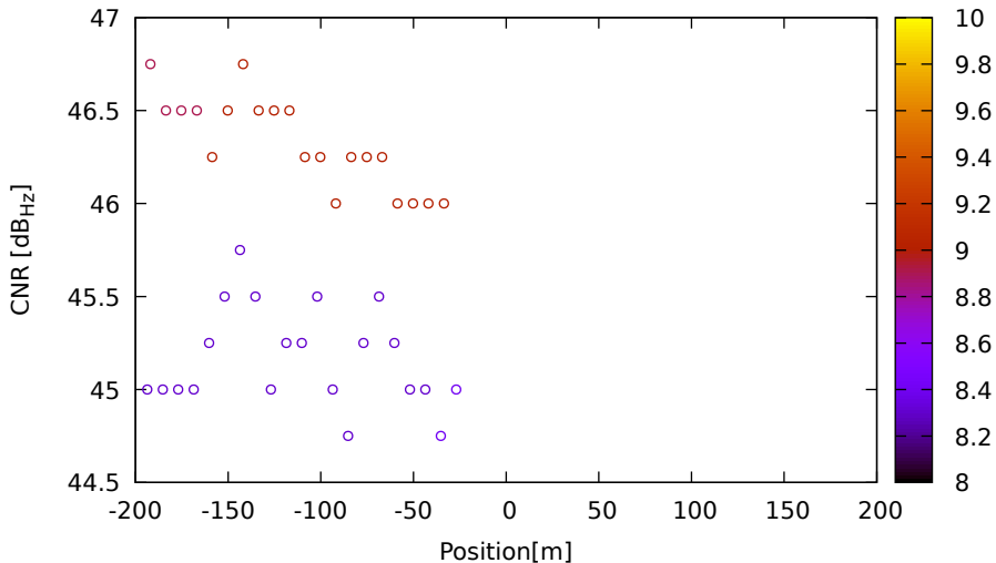
CNR vs position for E15 (E5b) on LeicaGS15 - DOY 262 jam. 3
