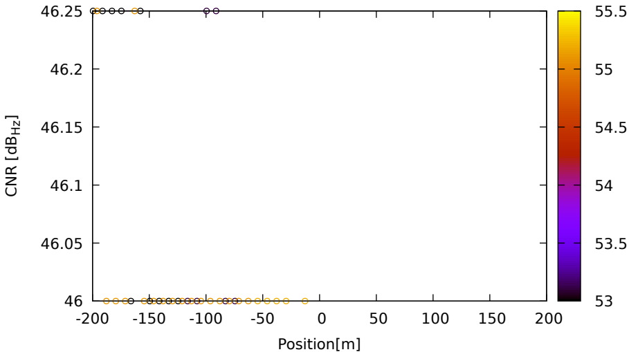
CNR vs position for E34 (E5) on LeicaGS15 - DOY 262 jam. 2
