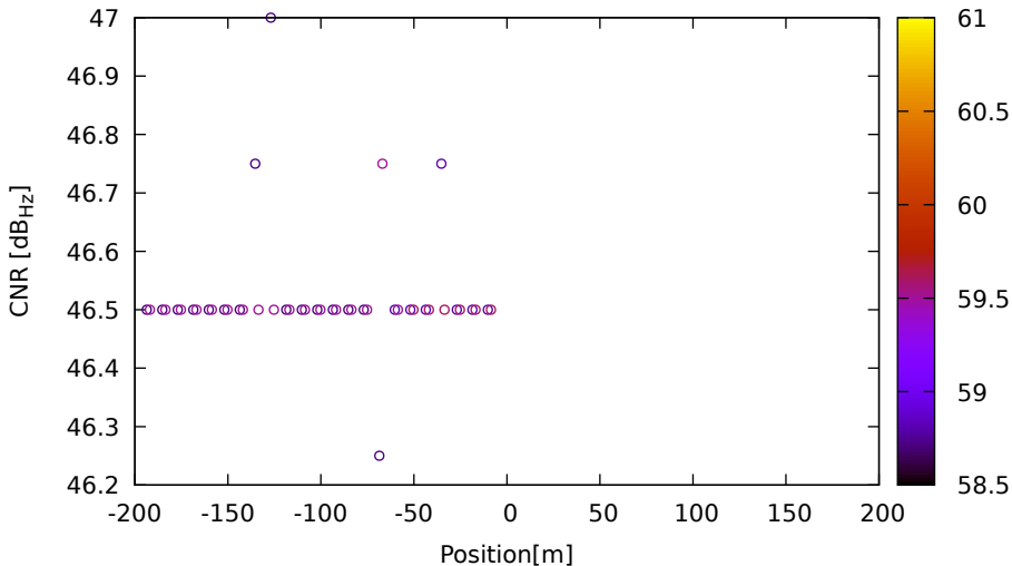
CNR vs position for E34 (E5) on LeicaGS15 - DOY 262 jam. 3
